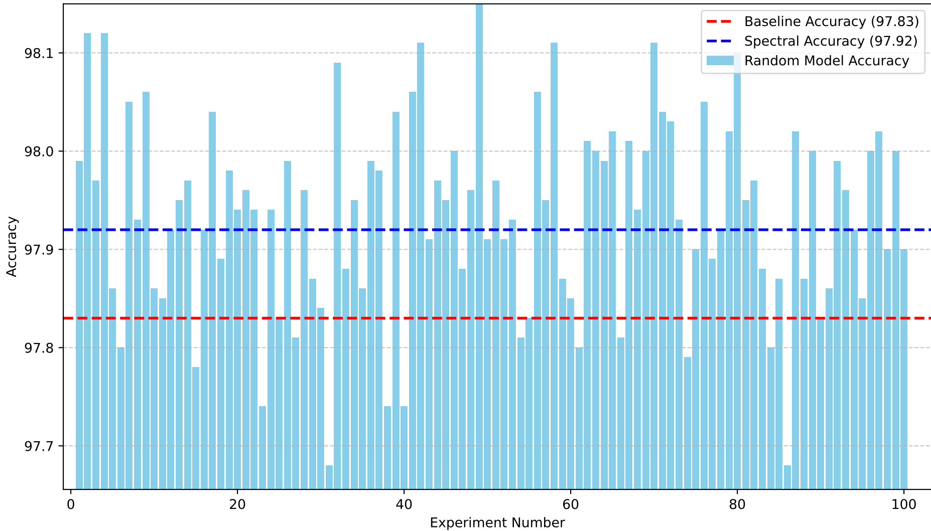
Accuracy vs Random Pruning
